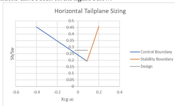
Figure 10. Horizontal Tailplane Sizing
