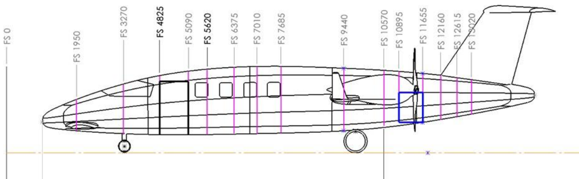
Figure 8. Fuselage structural layout
