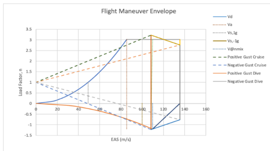
Figure 12. Flight Maneuver Envelope
