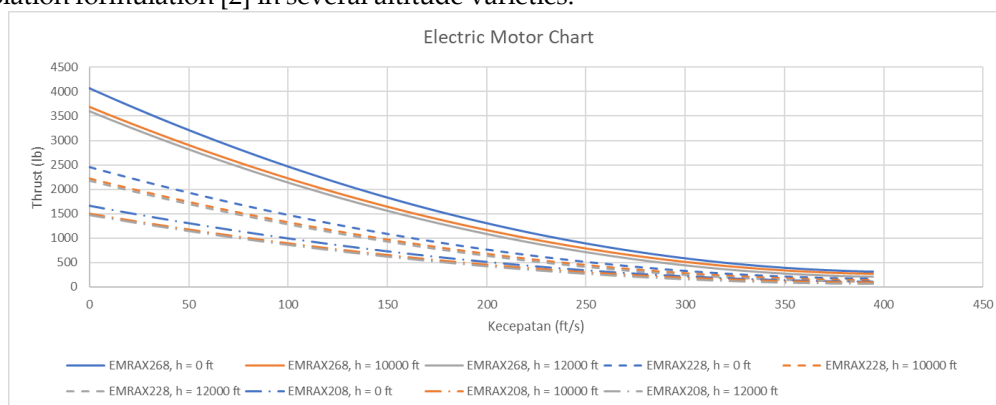
Figure 12. Electric Motor Chart
