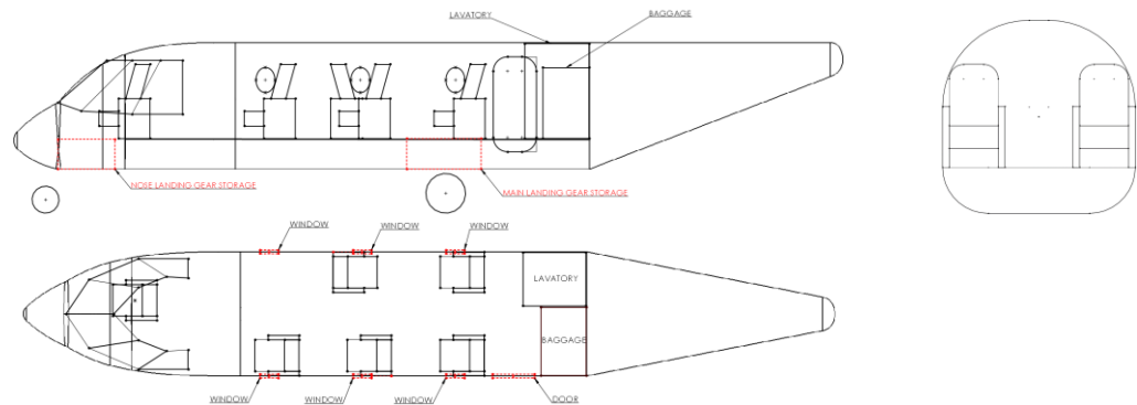
Figure 3. e-SPaRTA Fuselage Top View, Side View, and Cross-Section View
