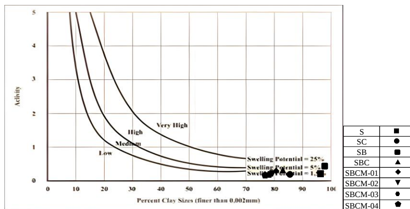
Figure 5. Graph of Activity Analysis Results with Variations in Matos Content and Curing 7 Days [8]
