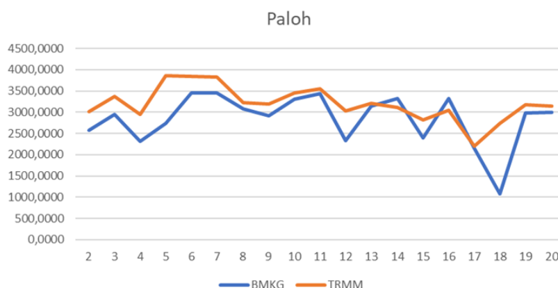
figure 5. Comparison of Annual Paloh Station Rainfall Data
