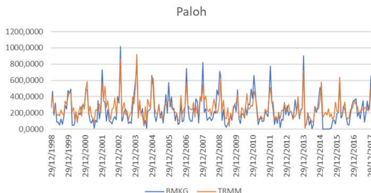
Figure 3. Comparison of 30-Day Paloh Station Rain Data
