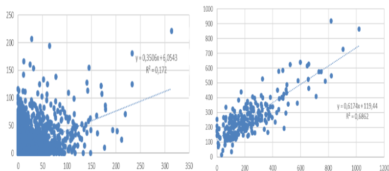
Figure 9. Correlation of BMKG and TRMM data for daily rainfall (left) and monthly (right)
