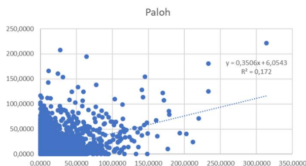
Figure 2. Daily Cumulative Paloh Station Linear Regression Graph
