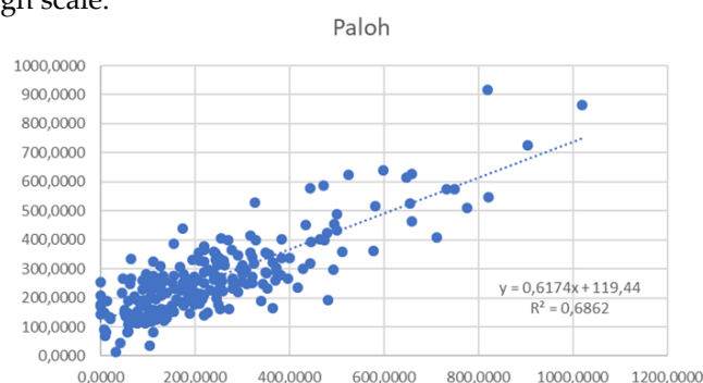
Figure 4. Linear Regression Graph Paloh Station Cumulative 30 Days
