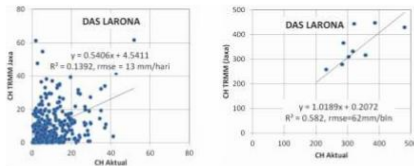
Figure 7. Correlation of TRMM rainfall data for daily (left) and monthly (right)
