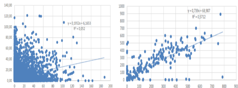
Figure 8. Correlation of BMKG and TRMM data for daily rainfall (left) and monthly (right)
