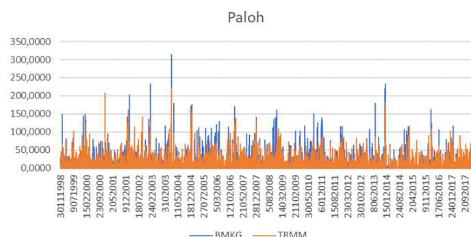
Figure 1. Comparison of Daily Cumulative at Paloh Station Rain Data
