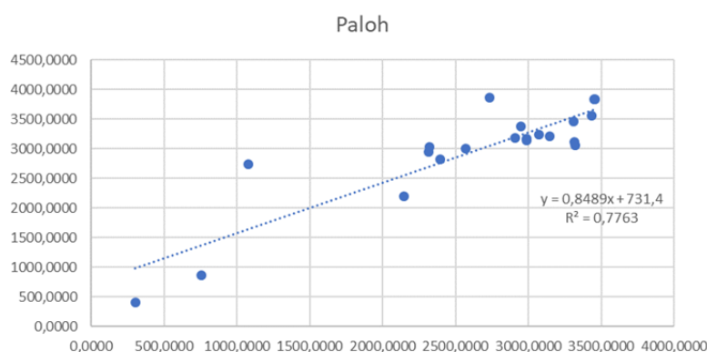
Figure 6. Annual Cumulative Paloh Station Linear Regression Graph
