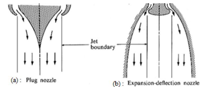
Figure 1. Type of plug nozzle geometry
