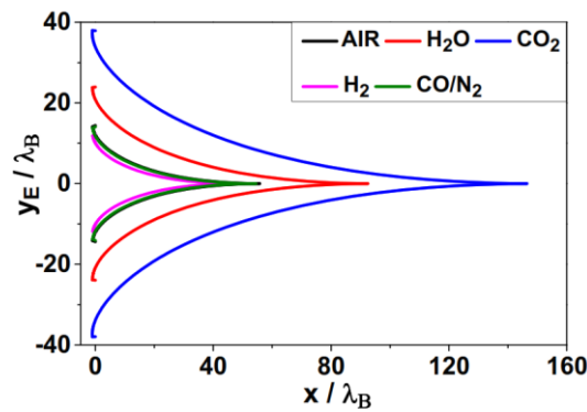
Figure 9. Gas effect on the plug shape giving ME=5.00 and T0=2000 K
