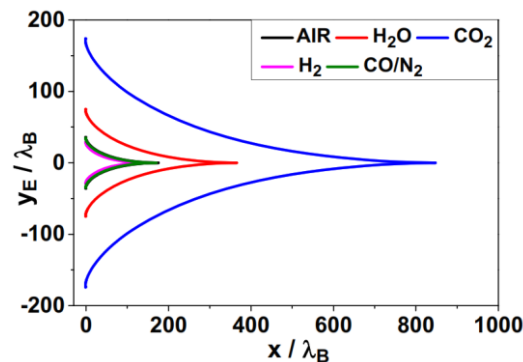
Figure 10. Gas effect on the plug shape giving ME=5.00 and T0=2000 K
