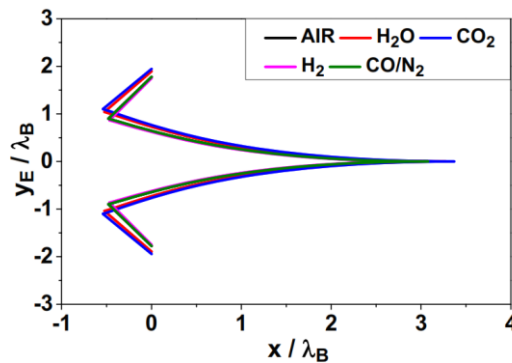
Figure 7. Gas effect on the plug shape giving ME=2.00 and T0=2000 K
