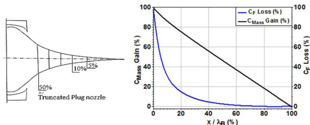
Figure 11. Representation of the gain in mass and the CF loss of a truncated 2D Plug nozzle for ME=3.00 and T_0=2000 K
