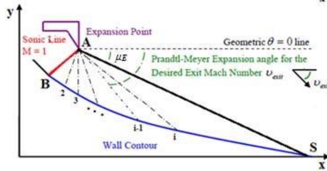
Figure 2. Generic geometry of a 2D plug Nozzle
