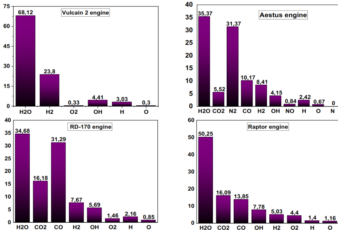
Figure 6. Examples of combustion products (%) of the various engines
