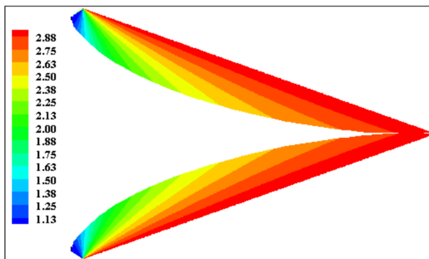
Figure 5. Profile and mesh of the nozzle for ME=3.00 and T_0=2000 K
