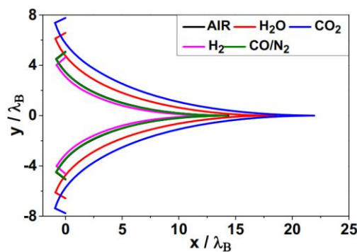
Figure 8. Gas effect on the plug shape giving ME=3.00 and T0=2000 K
