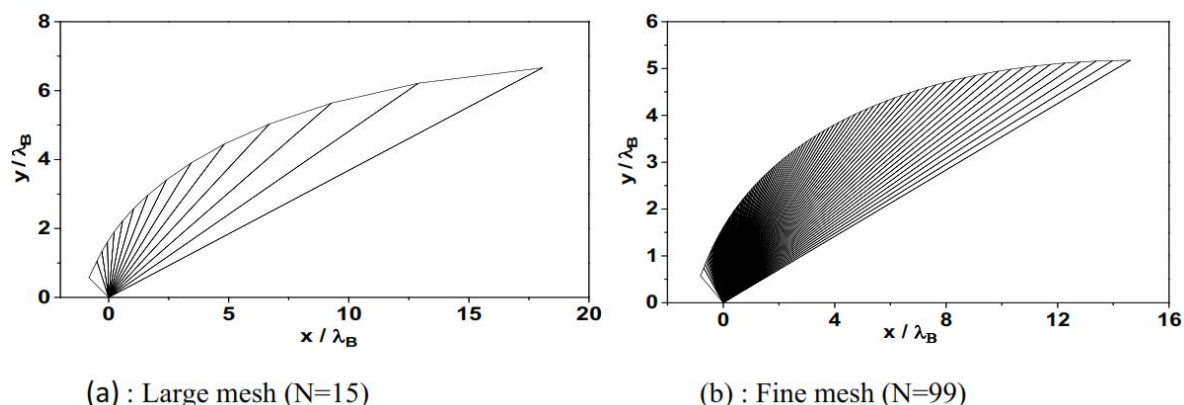
Figure 4. Contour nozzle and mesh of the nozzle for ME=3.00 and T_0=2000 K
