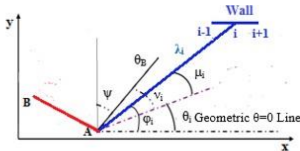
Figure 3. Geometric relationship between Mach lines and flow direction
