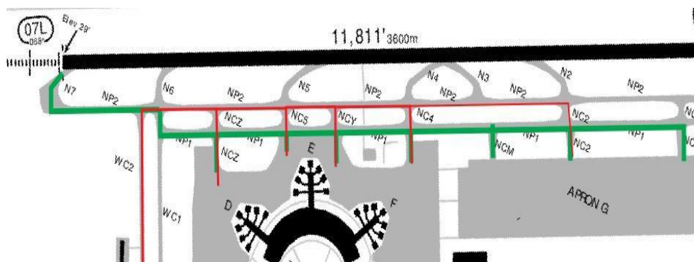
Figure 5. Improved taxiing route path at Soekarno-Hatta Intl Airport's north side
